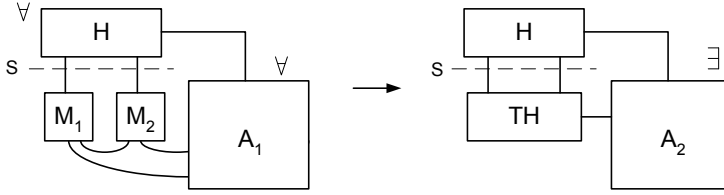
Fig. 3 Simulatability: The two views of H must be indistinguishable.
